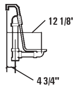
Rough-In Plumbing Measurements
