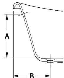
Drain/Overflow
